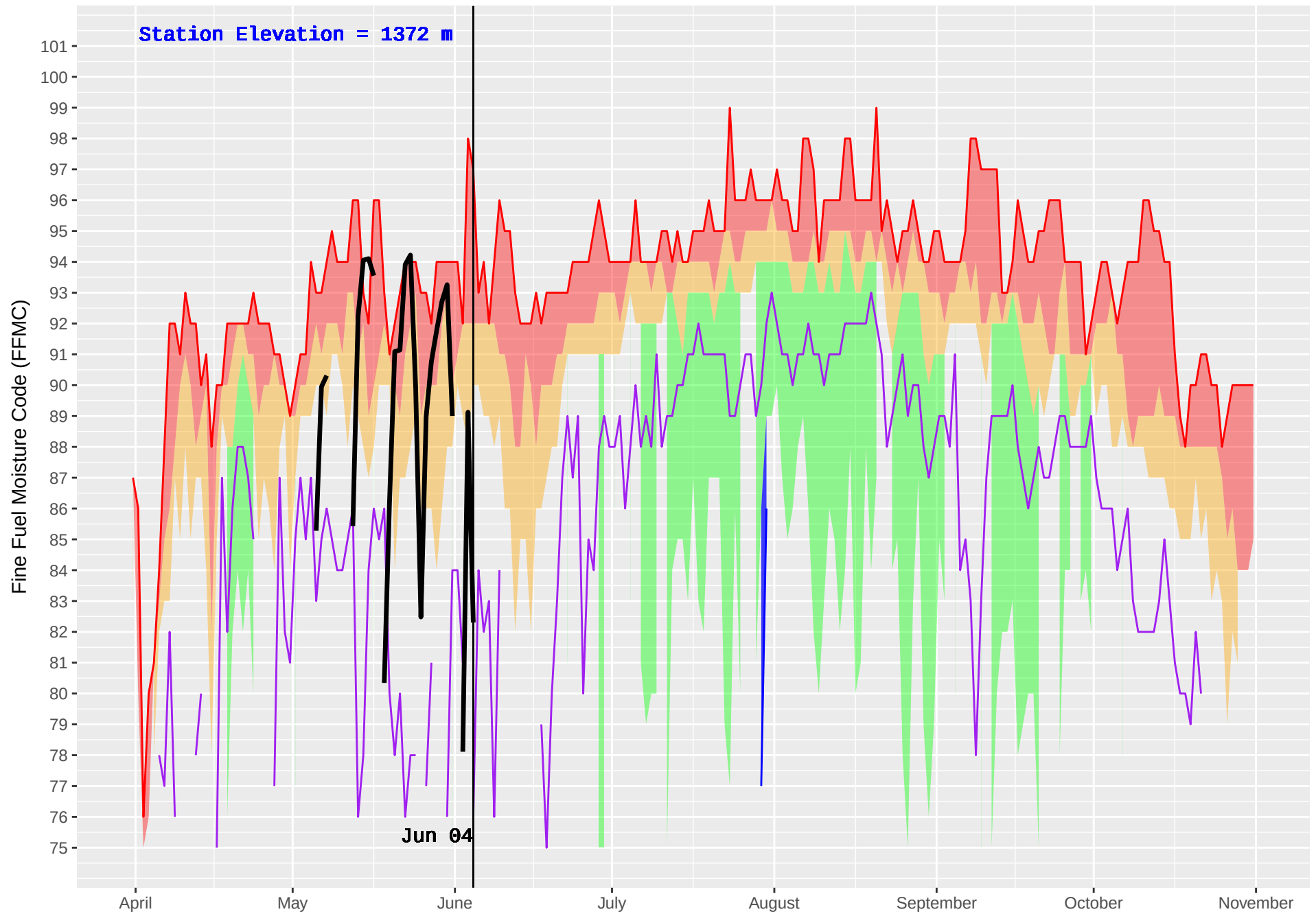
CHERRY LAKE (791) : Historical (1989–2016) and Current (2018) Noon Fine Fuel Moisture Code (FFMC)
