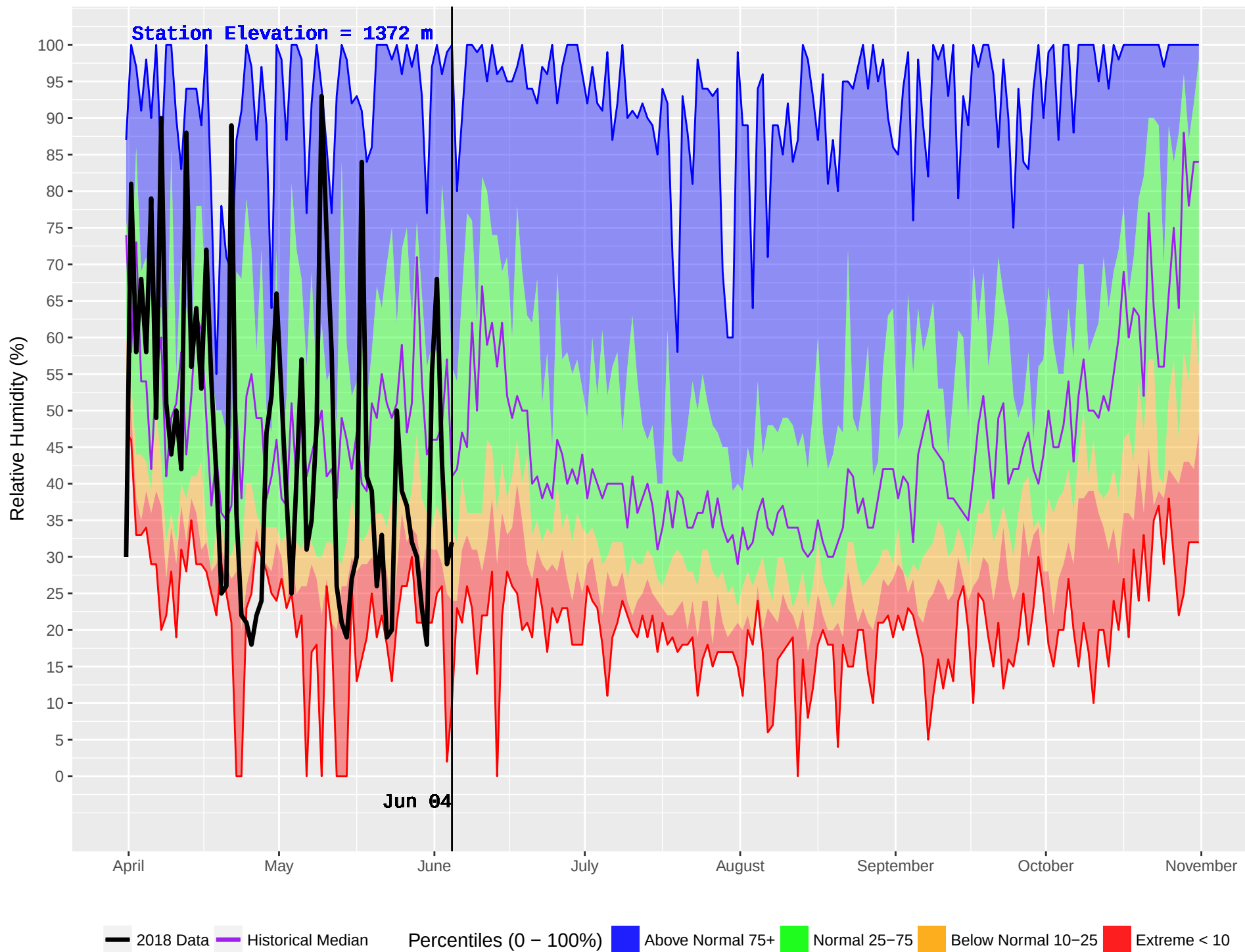
CHERRY LAKE (791) : Historical (1989–2016) and Current (2018) Noon Relative Humidity
