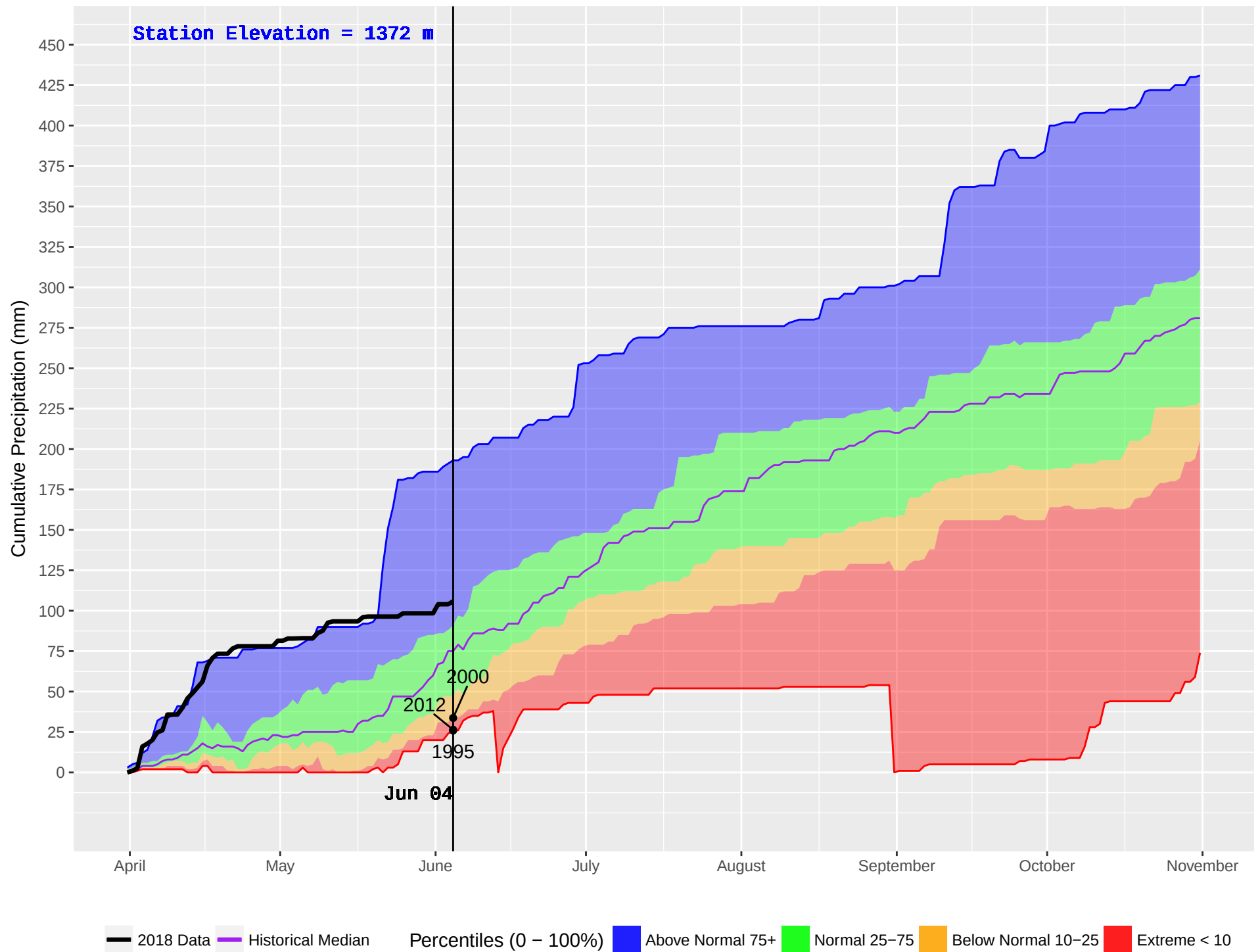
CHERRY LAKE (791) : Historical (1989–2016) and Current (2018) Noon Cumulative Precipitation
